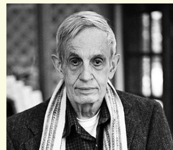
John Nash (1928 - )
