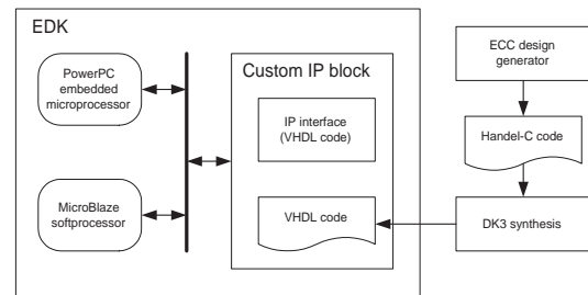
Figure 5. Diagram of the design flow.
