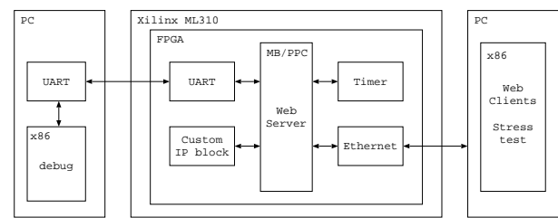
Figure 10. Secure web server overview.
