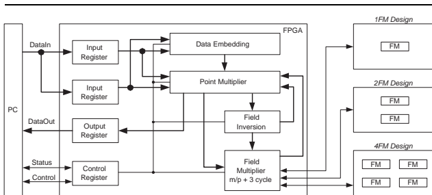
Figure 4. Datapath of the customisable ECC system.
