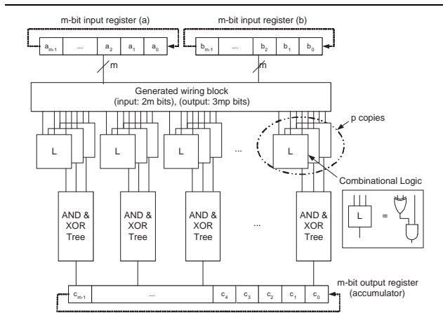
Figure 3. Parallel field multiplier IP block.
