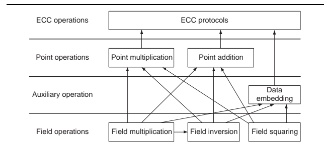
Figure 2. Interactions between different operations.
