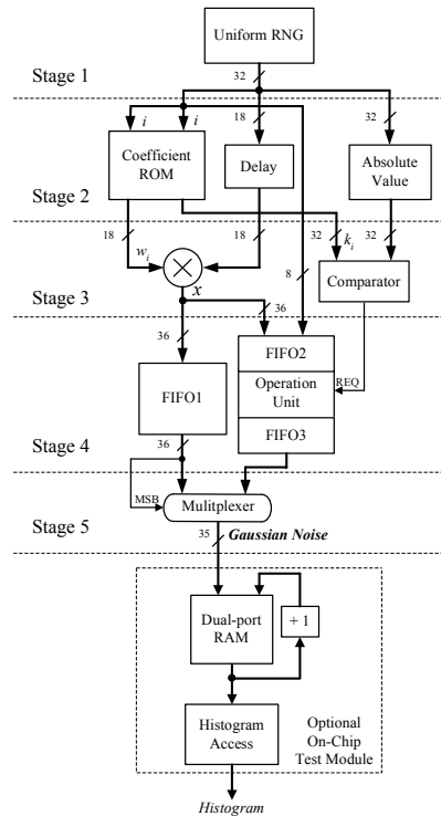
Fig. 1. Block diagram showing the architecture of the GRNG with optional on-chip test module. Horizontal dashed lines indicate pipeline registers and the bit-width of each bus is also shown.
