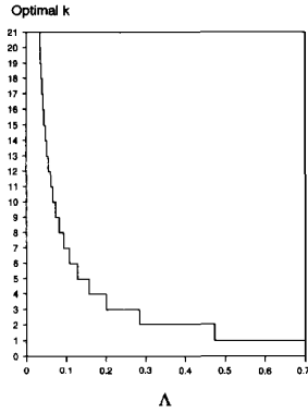
Fig. 3. Optimal multi-copy policy under different \Lambda .
