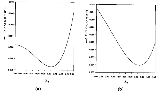
Fig. 2. Comparison of pure and mixed policies: (a) \lambda_1 + \lambda_2 = 0.5 , (b) \lambda_1 + \lambda_2 = 0.45 .
