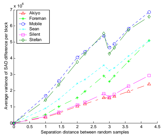
Fig. 3 Variance of block SAD difference for the random sample pairs taken from the 4x4 region around the global minimum
