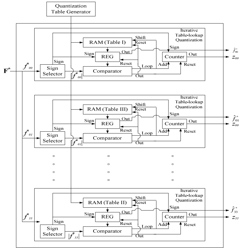
Fig. 3. Hardware architecture for iterative table-lookup quantization process
