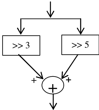
Fig. 5 Architecture of shifter for region III
