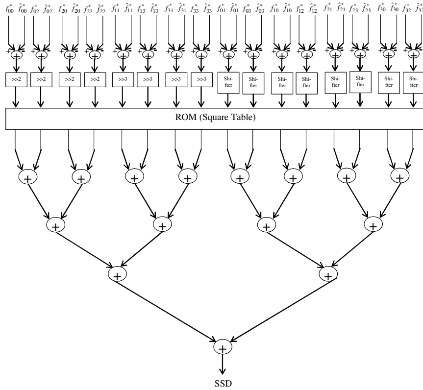
Fig. 4. Architecture of SSD calculator
