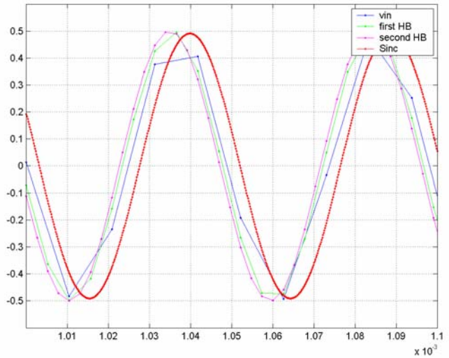
Figure 9. Interpolator Curve.
