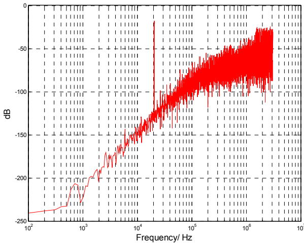
Figure 5: DAC output spectrum with the 3 rd order setting.
