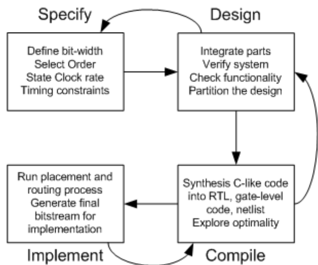
Figure 7. Design Process.
