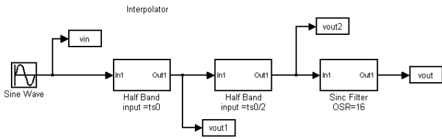
Figure 8. Interpolator Architecture.
