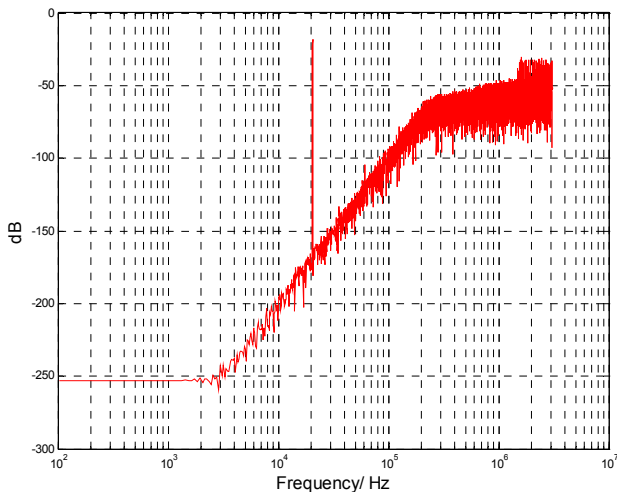
Figure 6: DAC output spectrum with the 5 th order setting.
