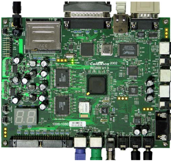
Figure 14. Photograph of the Celoxica RC200 board
