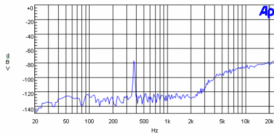
Figure 24. Audio-Precision Measurement 2
